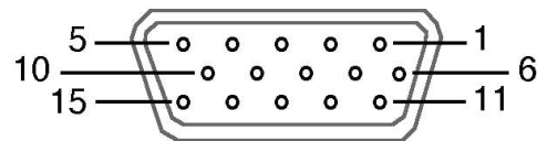
ACC Connector (female, on KIO3 panel, viewed from the back of the K3)
