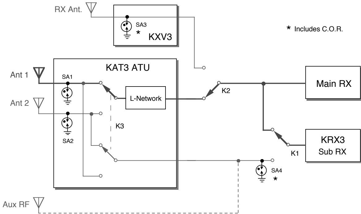
Figure 4. Main/Sub Receiver Routing with KXV3 and KAT3 Installed
